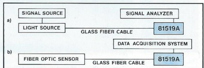
The HP 81519A Optical Receiver can operate either as a front-end interface to conventional test equipment (a) or as a precision interface to measurement or process control systems (b).
