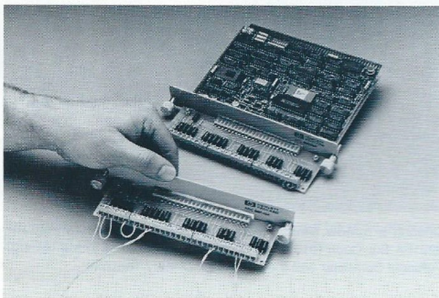
The HP 98640A Analog Input Interface is an easy-to-use data acquisition tool for the HP 9000 Series 200 Computers. This modular board features a screw termination assembly, which can be unfastened and replaced by another assembly instead of rewiring.
