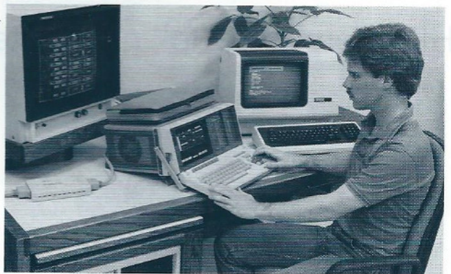
An advanced network management tool, the HP 4953A Protocol Analyzer can monitor performance and simulate data-terminal equipment or data-circuit terminating equipment to find hard-to-spot errors that can make your network go down. The HP 4953A can also verify system components before they are installed in your network.
