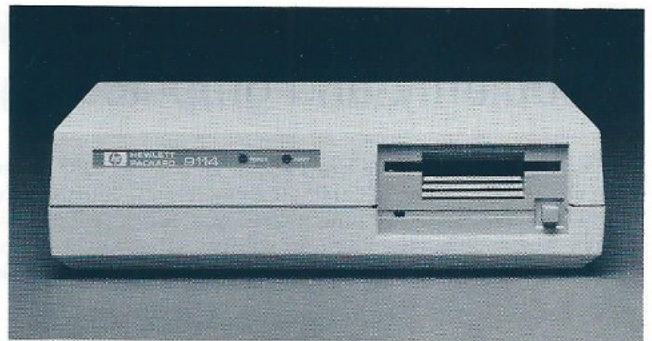
This new lightweight, portable disc drive offers 710 kbytes of formatted capacity. It is compatible with HP and IBM personal computers and HP's handheld calculators and computers.
