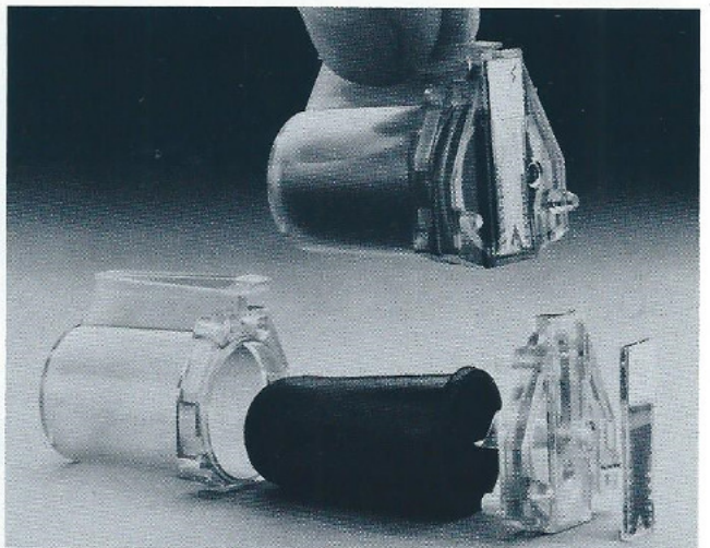
This disposable ink-jet printhead used in the HP ThinkJet printers holds about 3 cc of usable ink, enough to print about 500 pages of text. Thanks to its see-through design, you can see how much ink is left so you can replace the cartridge before the ink runs out.
