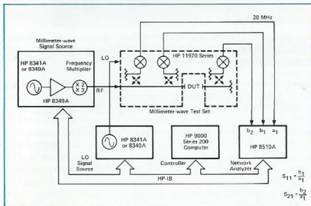
This simplified block diagram shows a millimeter-wave network analyzer based on the HP 8510A analyzer.
