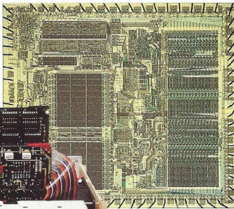
The Motorola MC68000 chip, the "heart" of the HP 9836A, is a state-of-the-art 16-bit microprocessor.
