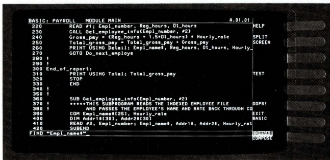
Fig. 5. The IDS screen while the BASIC language subsystem is in command mode.
