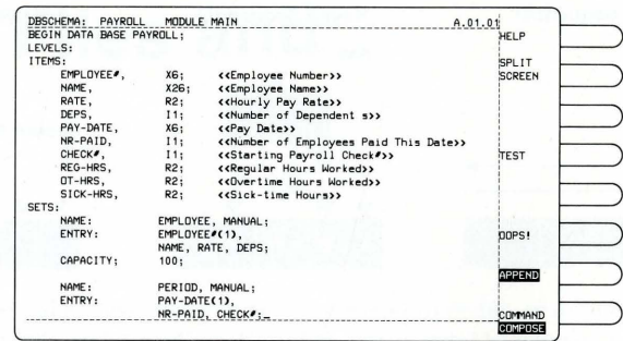
Fig. 4. Entering the schema that describes the structure of the data base of Fig. 3.
