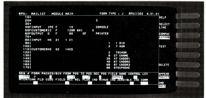
Fig. 4. Editing a previously entered line using the APPEND/MODIFY, SELECT LINE, and DELETE softkeys.
