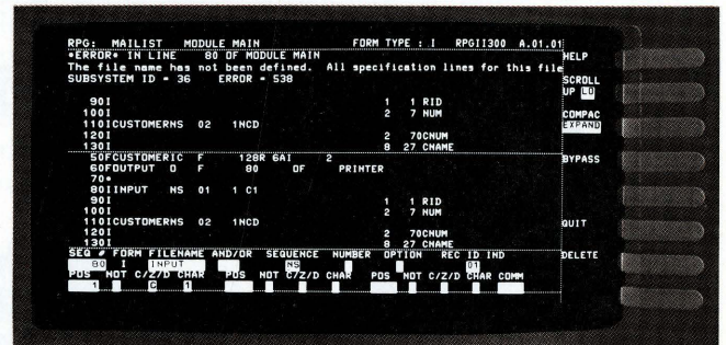
Fig. 5. When the TEST softkey is pressed, compilation begins. If an error is discovered, it is displayed on a split screen. The user can correct the error, BYPASS it temporarily, or QUIT the error processing mode.
