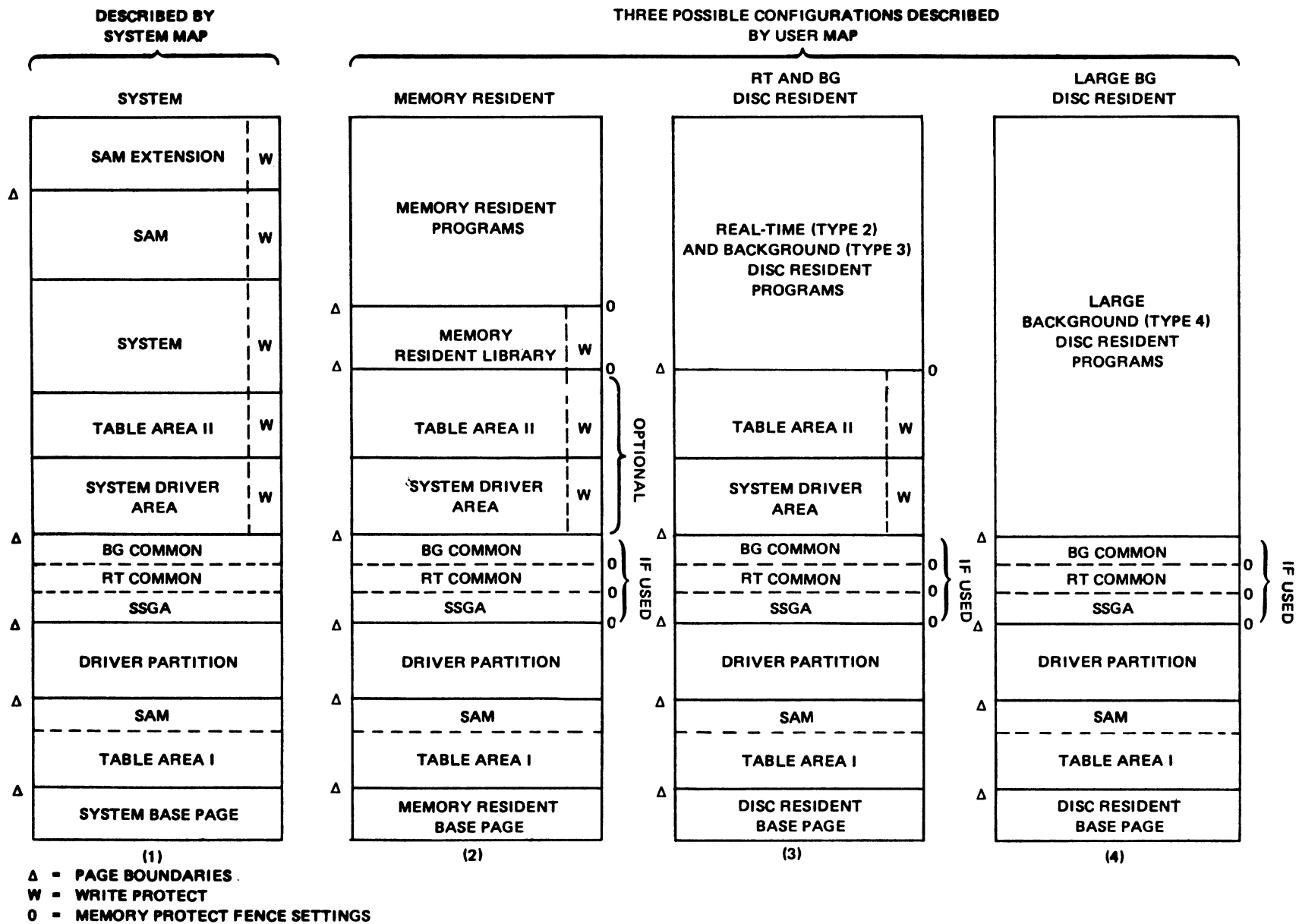
Figure B-2. RTE-IVB 32K Logical Memory Configurations
