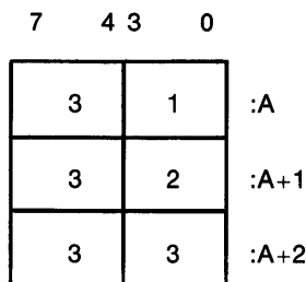
Zoned Format or Unsigned
