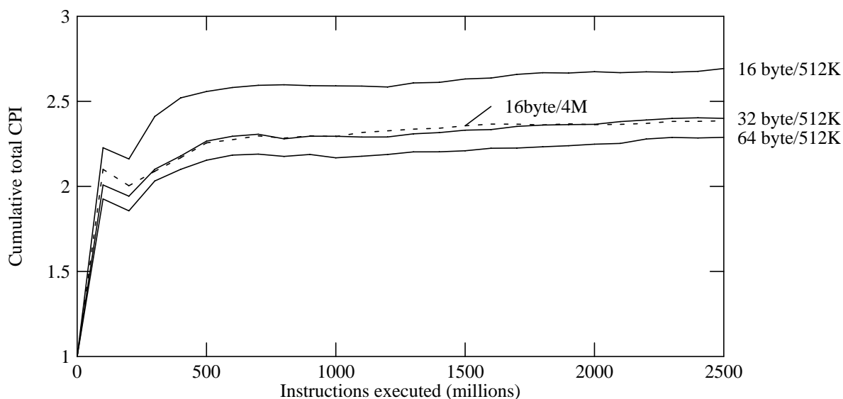
Figure 17: Three line sizes for the first level caches
