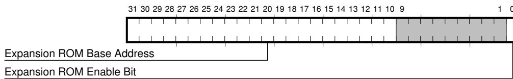
Figure 3–8 CBER Expansion ROM Base Address Register
