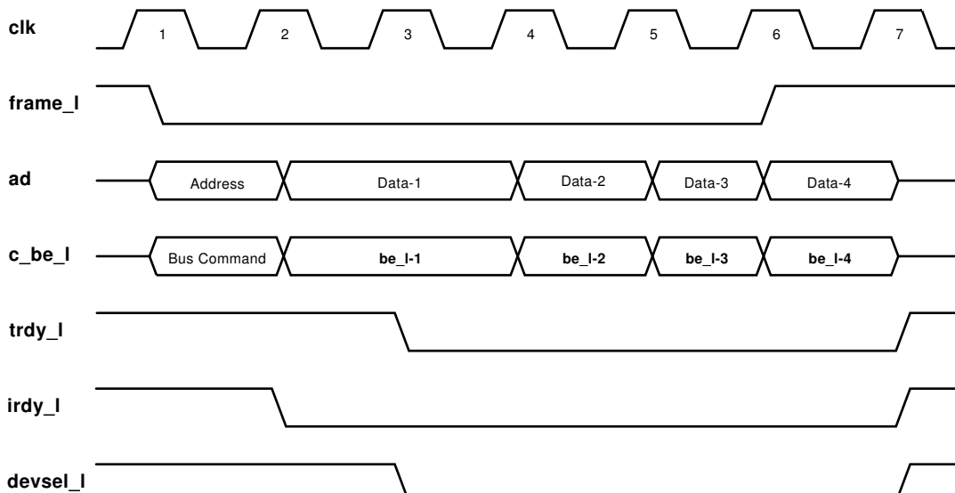
Figure 5–6 Memory Write
