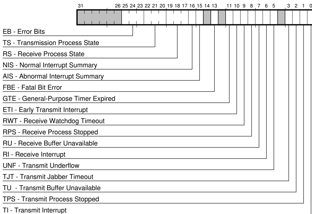
Figure 3–16 CSR5 Status Register
