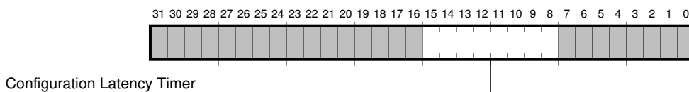
Figure 3–4 CFLT Configuration Latency Timer Register
