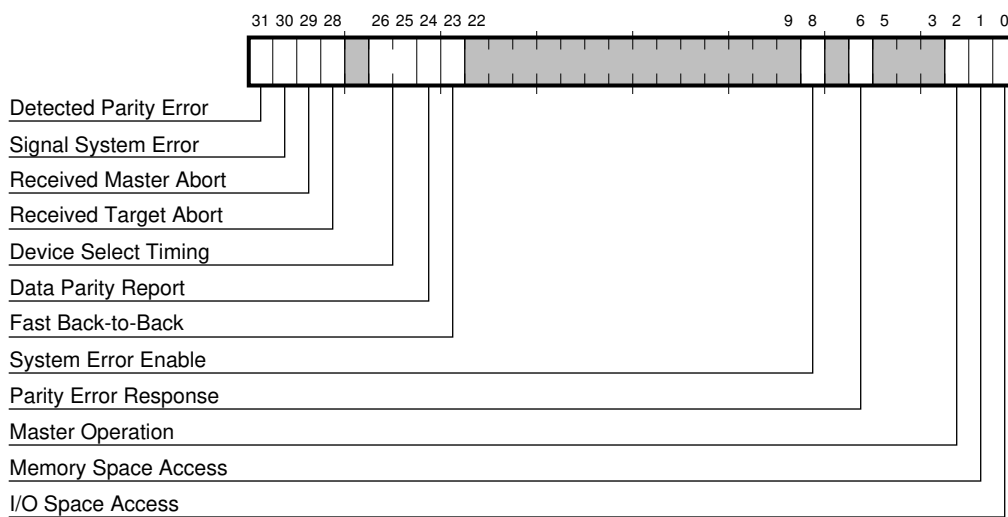
Figure 3–2 CFCS Command and Status Configuration Register
