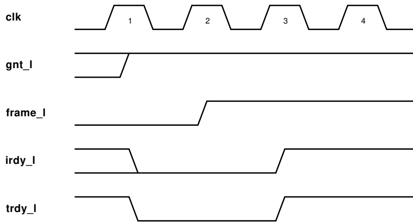
Figure 5–8 Normal Completion
