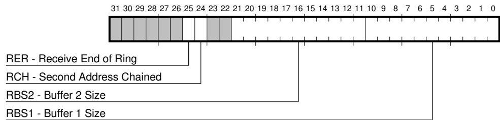
Figure 4–4 RDES1 Receive Descriptor 1
