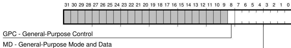
Figure 3–23 CSR12 General-Purpose Port Register
