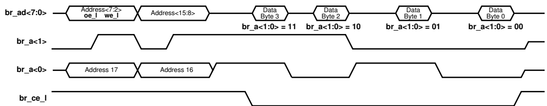
Figure 7–4 Boot ROM Dword Read Cycle
