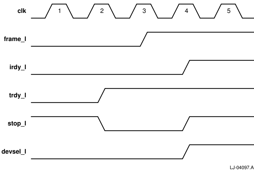
Figure 5–12 Target Retry
