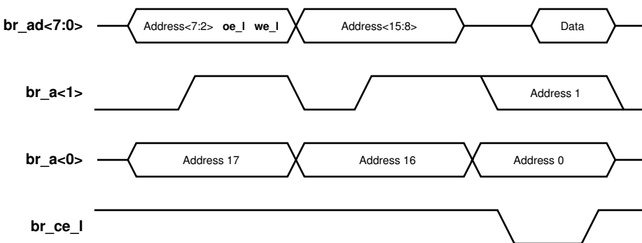
Figure 7–2 Boot ROM Byte Read Cycle
