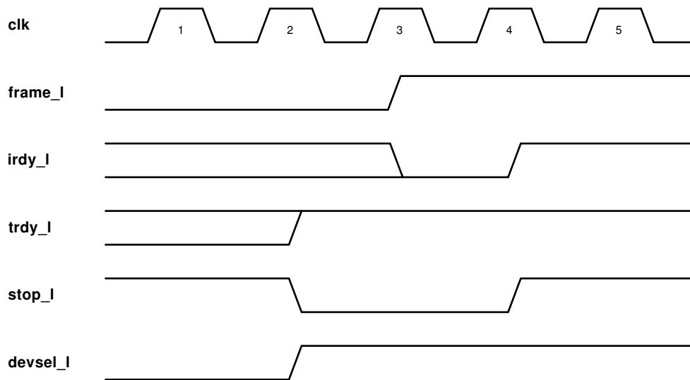
Figure 5–10 Target Abort
