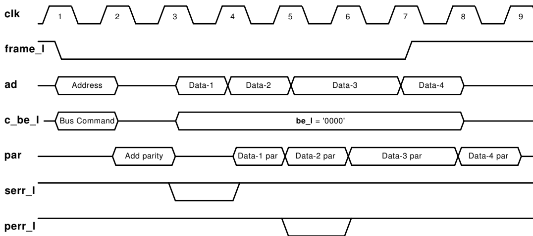
Figure 5–13 Parity Operation
