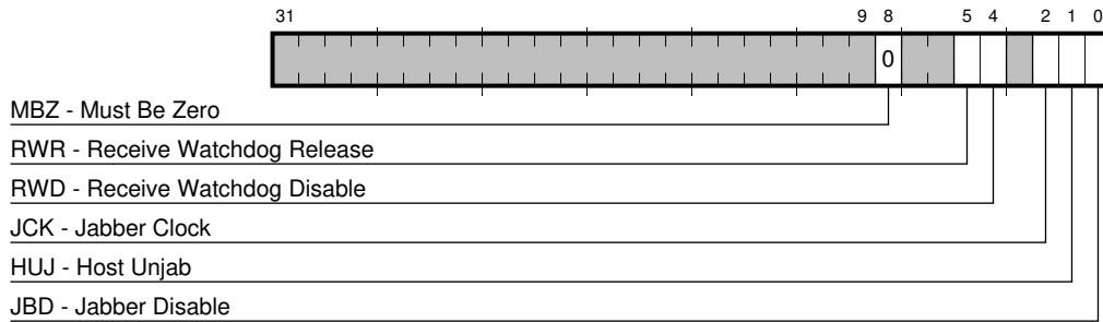
Figure 3–24 CSR15 Watchdog Timer Register
