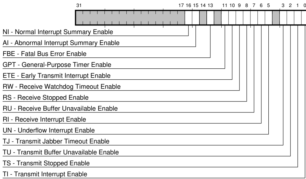
Figure 3–18 CSR7 Interrupt Enable Register
