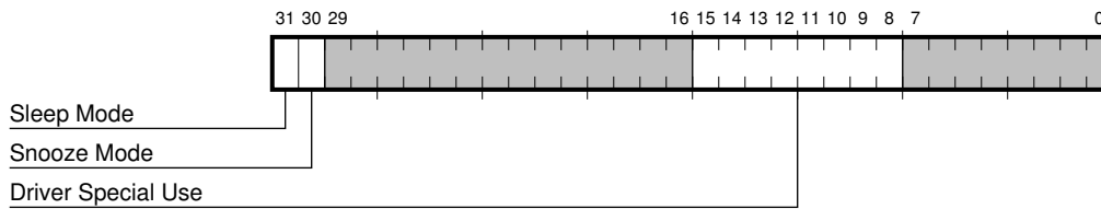
Figure 3–10 CFDD Configuration Driver Area Register
