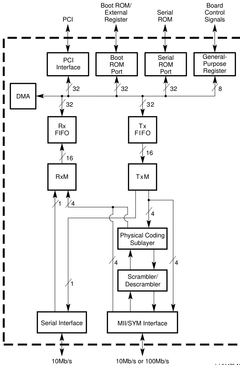
Figure 1-1 21140A Block Diagram
