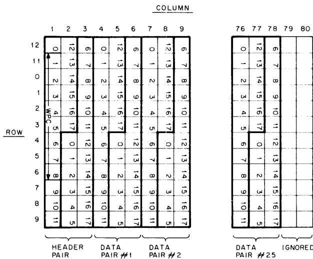
Figure 4-1 IOPS Binary Input Card Format
