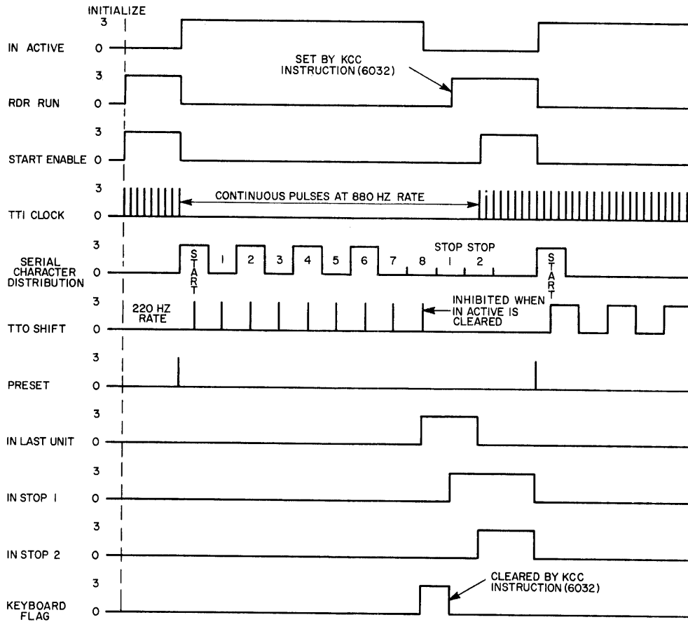
Figure 4-2 Teletype Read Cycle Timing Diagram
