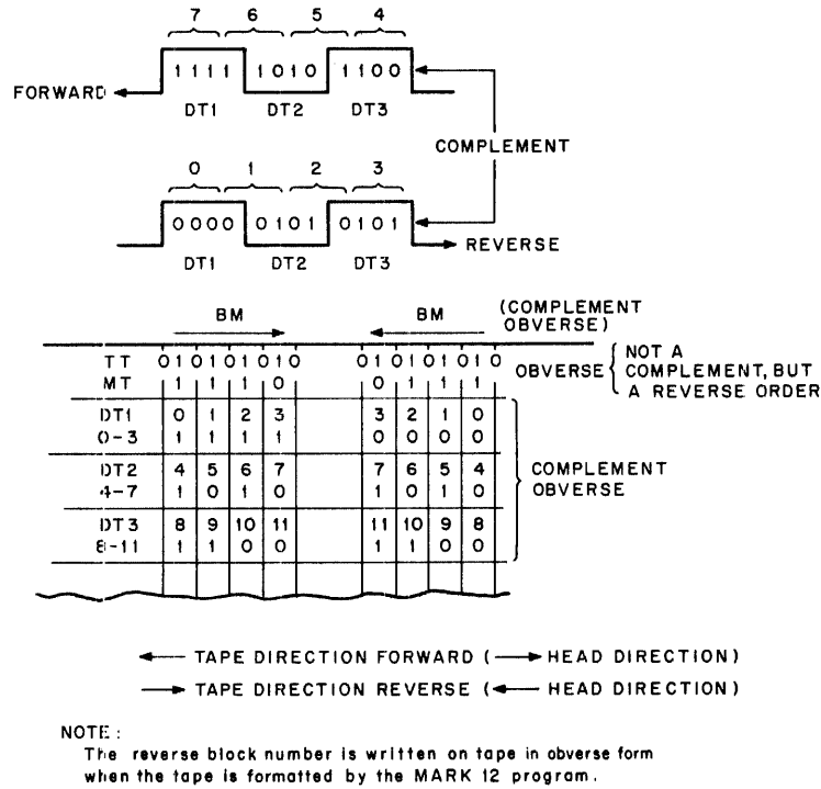
Figure 6-14 Reading A Block Mark
