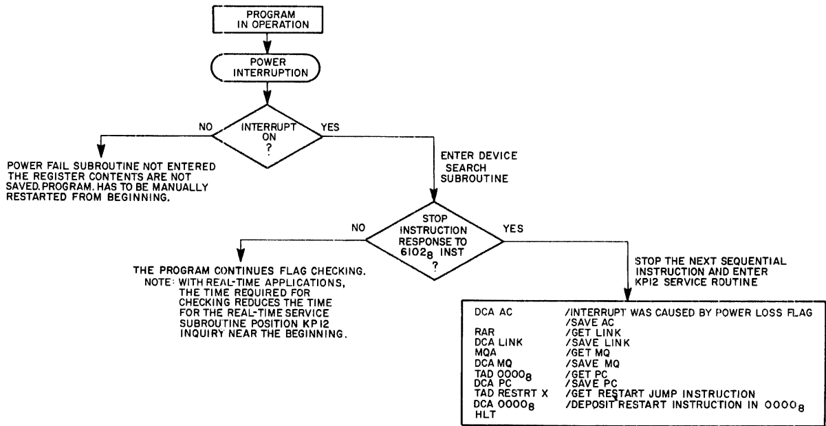
Figure 7-8 Automatic Restart Program Events
