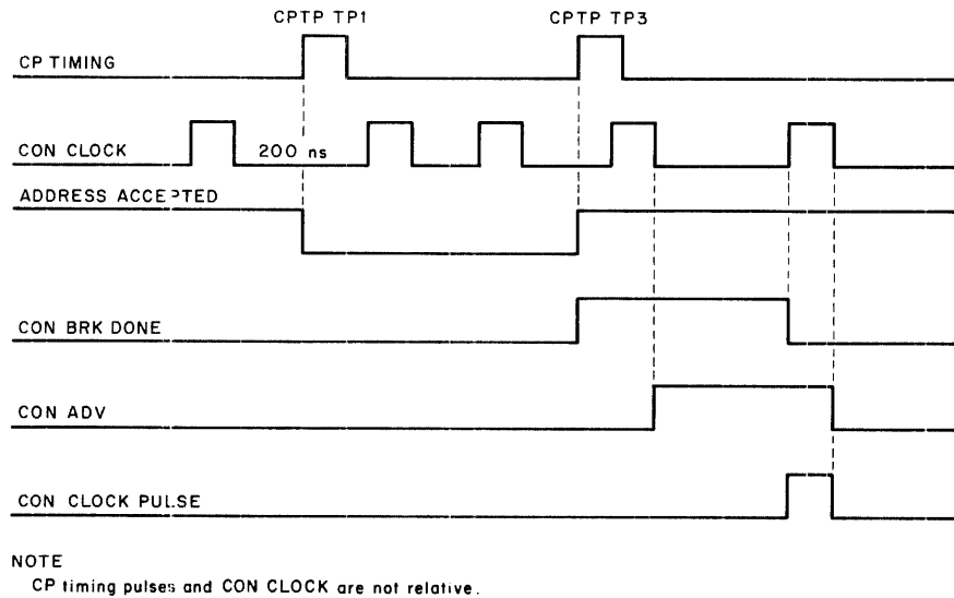
Figure 7-6 Control Timing
