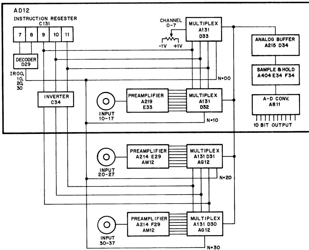
Figure 7-1 Multiplexer Selection
