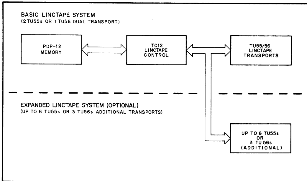
Figure 6-1 LINAtape System Configuration
