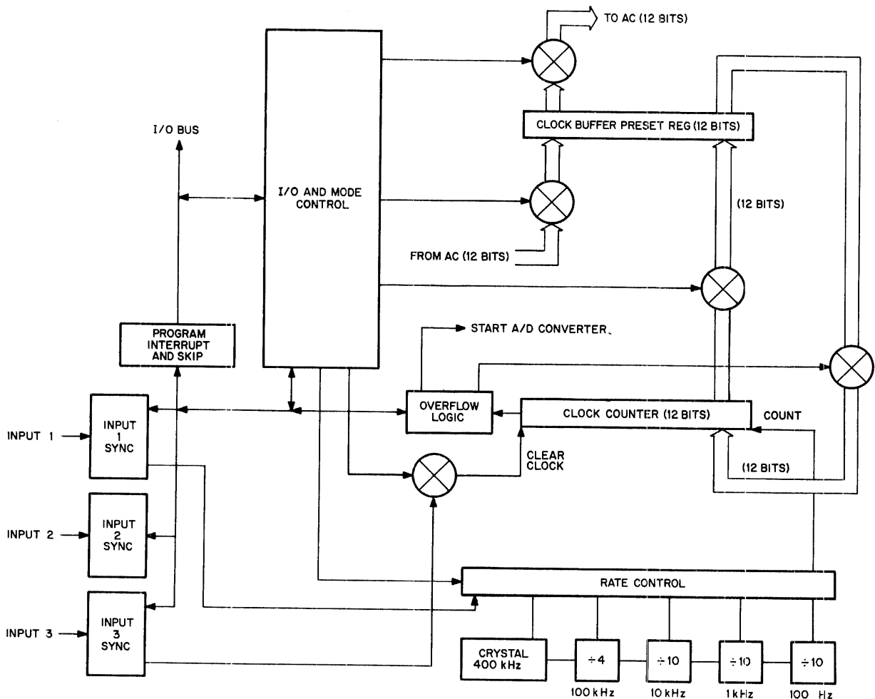
Figure 7-11 KW12-A Organization
