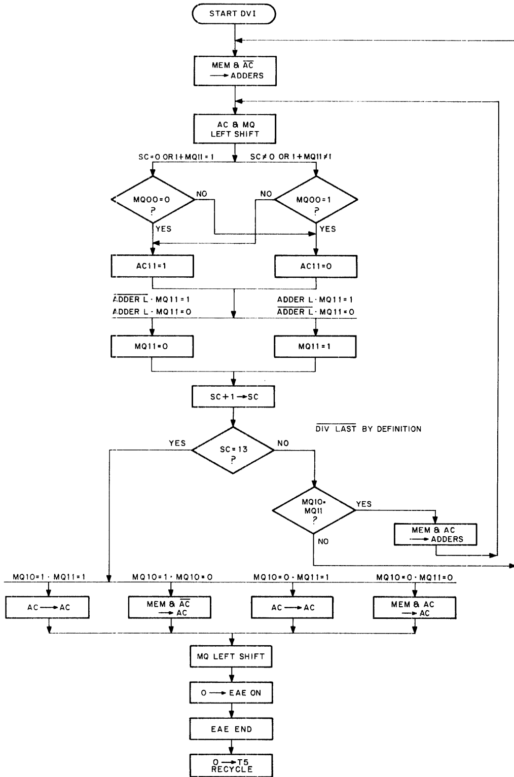
Figure 7-3 KE12 EAE DVI Flow Chart
