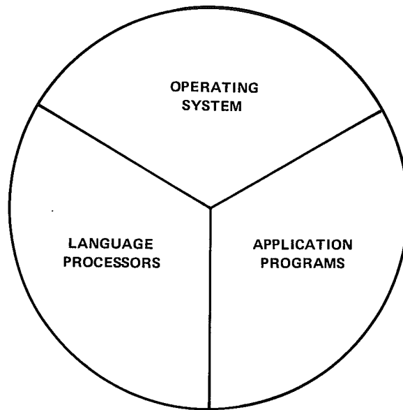
Figure 1-6 System Software
