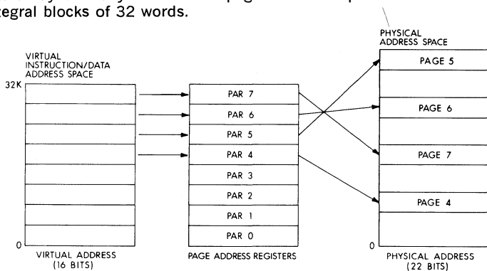
Figure 6-6 Virtual Address Mapping into Physical Address
