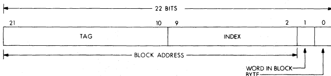
Figure 7-5 Physical Address
