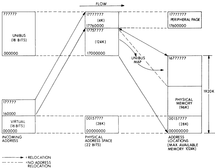
Figure 6-3 16 Bit Mapping
