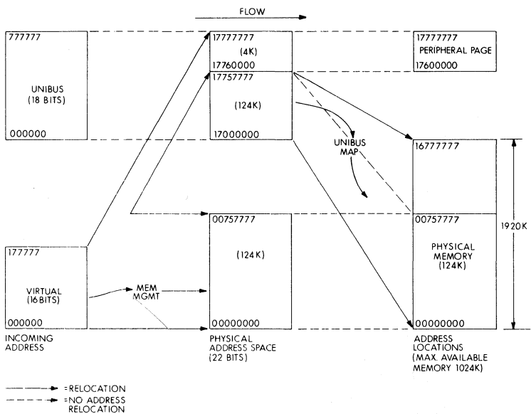
Figure 6-4 18-Bit Mapping
