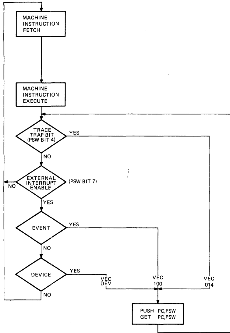
Interrupt and Trap Portion of Machine Cycle Figure 2-15
