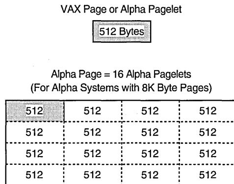
Figure 1-1 Comparison of VAX and Alpha Page Size
