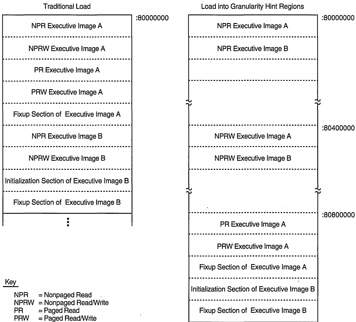
Figure 7-1 Traditional Loads and Loads into GHRs
