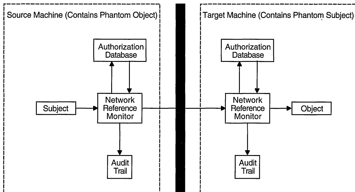
Figure 9-2 Advanced View of the Reference Monitor in a Network
