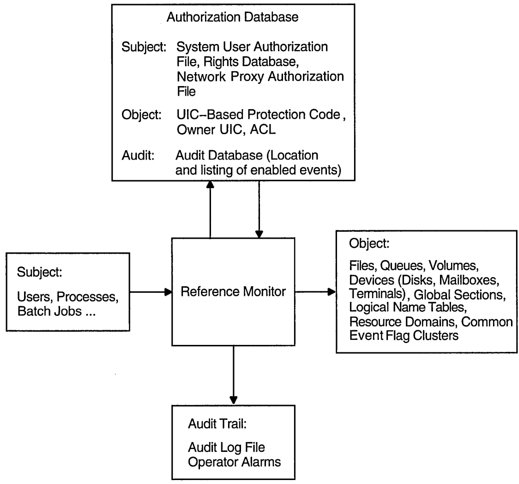
Figure 2-1 Reference Monitor
