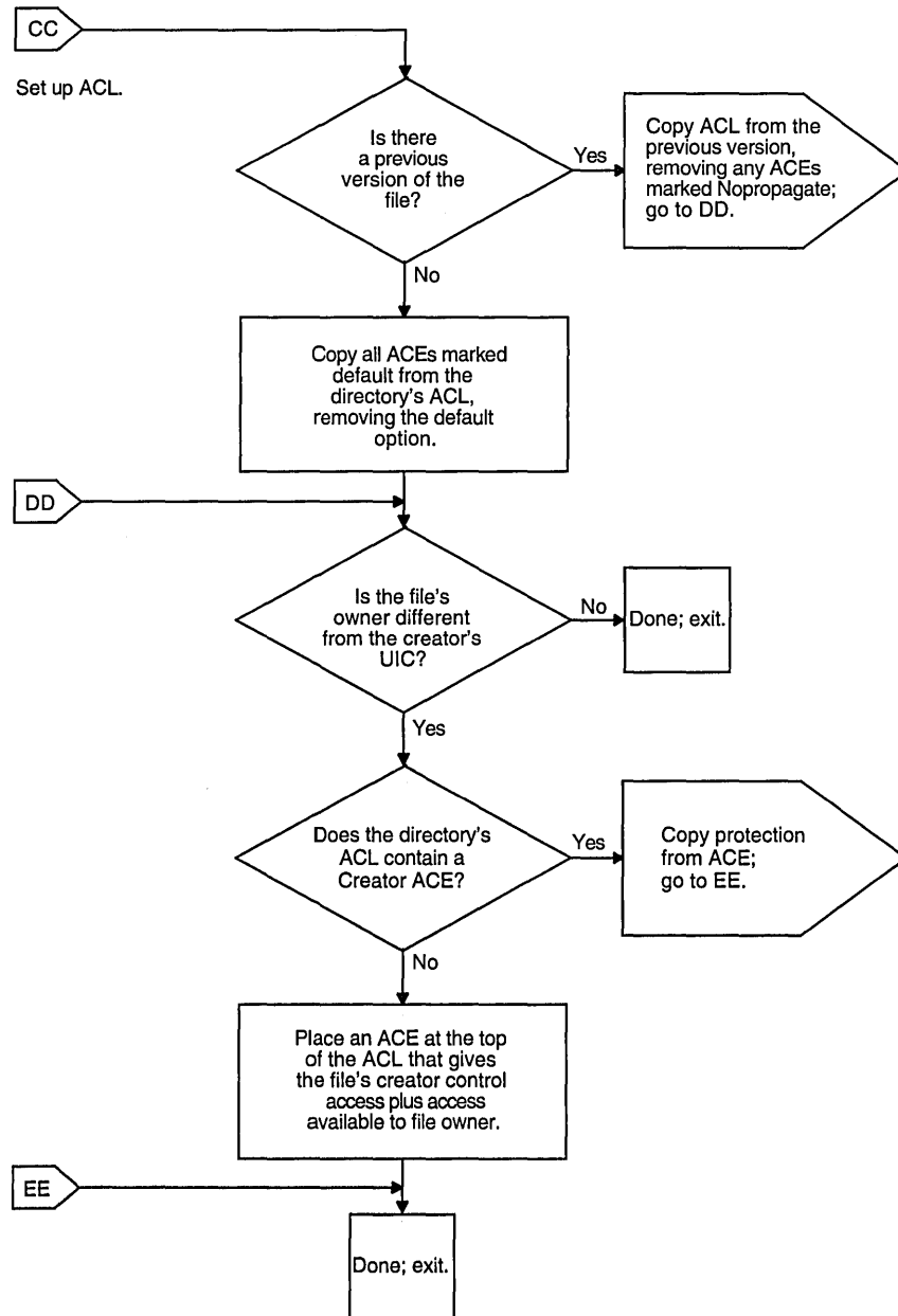
Figure 5-1 (Cont.) Flowchart of File Creation
