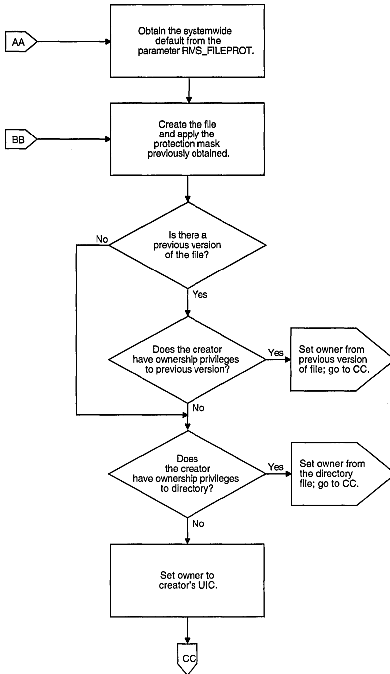
Figure 5-1 (Cont.) Flowchart of File Creation
