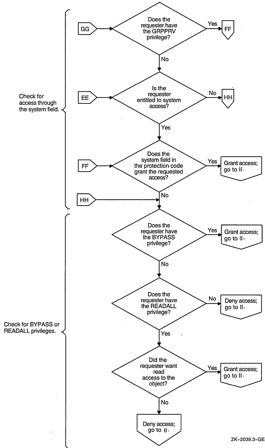
Figure 4-1 (Cont.) Flowchart of Access Request Evaluation
