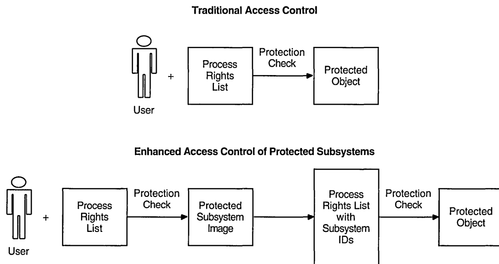
Figure 10-1 How Protected Subsystems Differ from Normal Access Control
