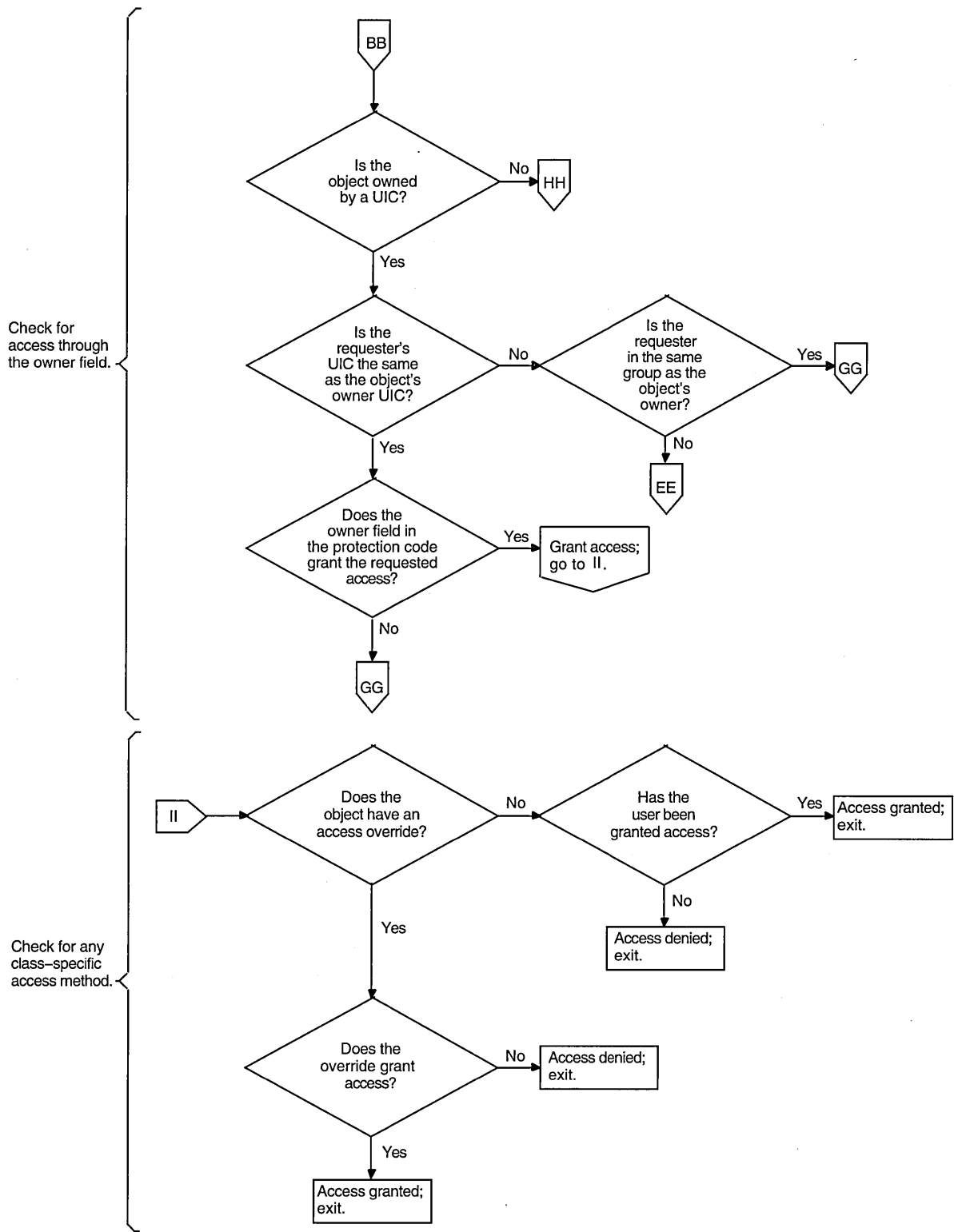
Figure 4-1 (Cont.) Flowchart of Access Request Evaluation
