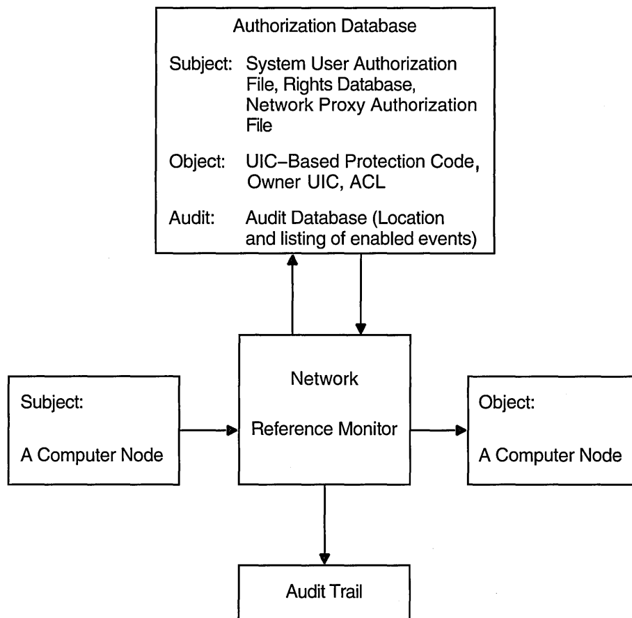
Figure 9-1 Simple View of Reference Monitor in a Network
