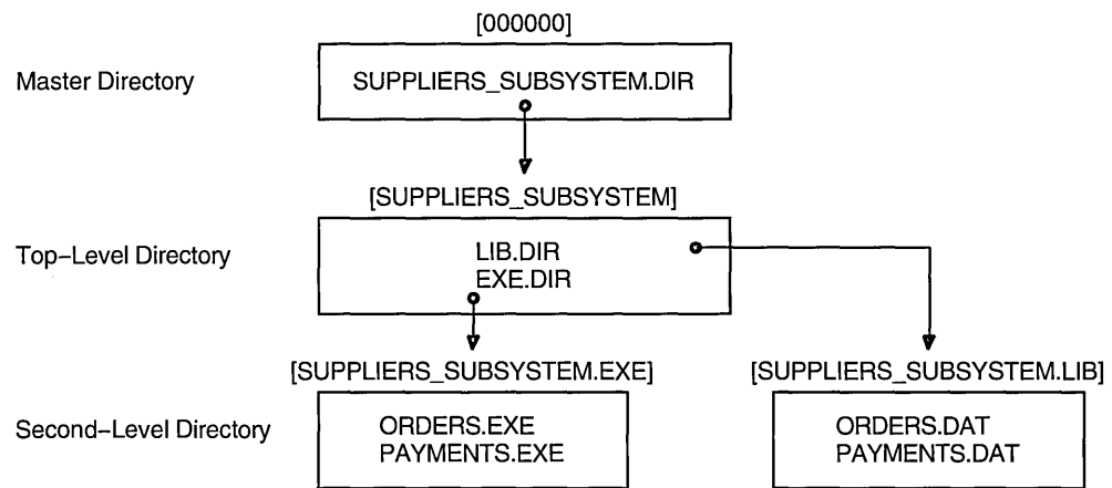
Figure 10–2 Directory Structure of the Taylor Company’s Subsystem
