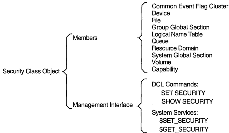
Figure 5-2 Security Class Object
