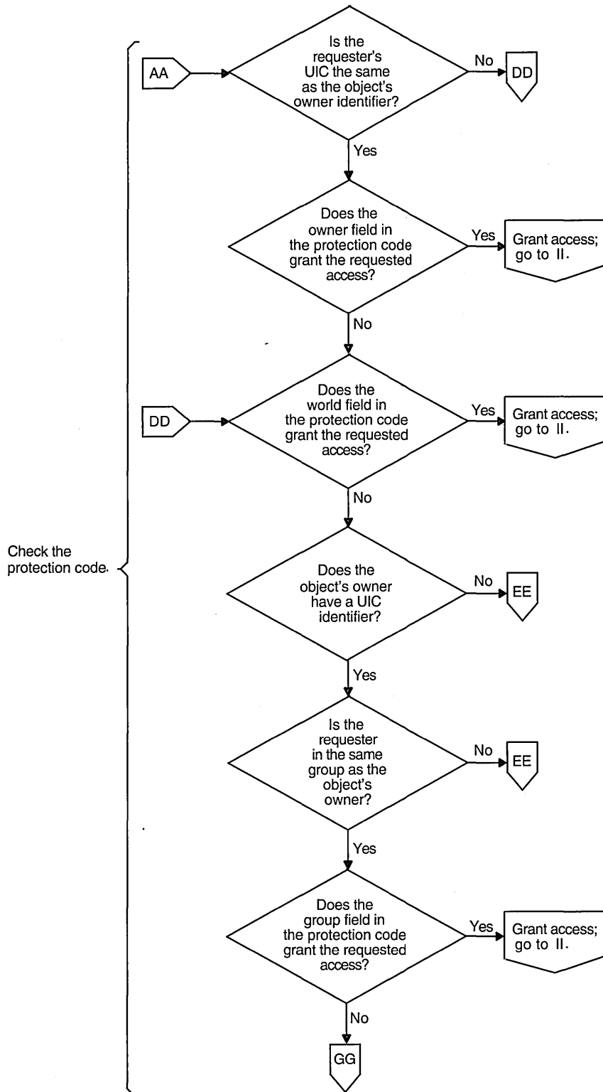
Figure 4-1 (Cont.) Flowchart of Access Request Evaluation
