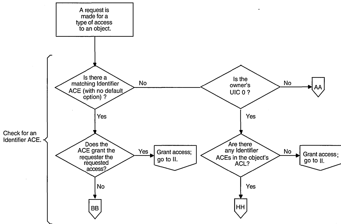
Figure 4-1 Flowchart of Access Request Evaluation
