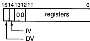
Figure 3.1 Procedure Entry Mask
