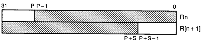
Variable-Length Bit Field Data Type across a Register Boundary
