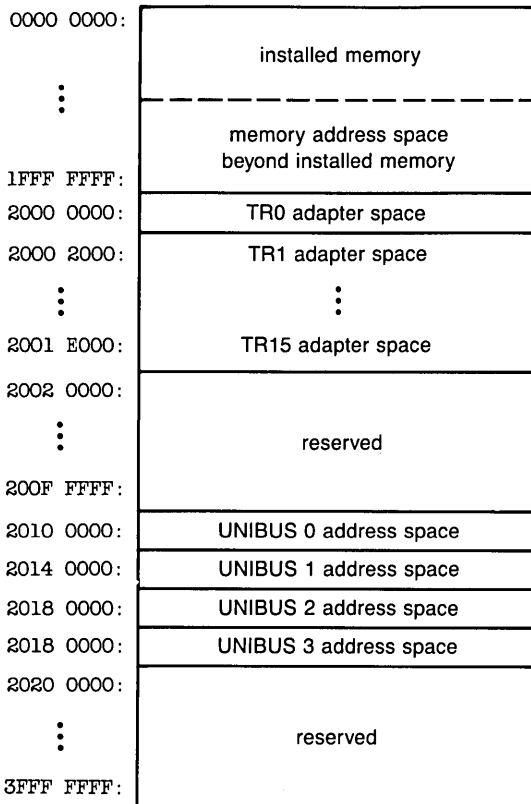
Figure B.13 VAX-11/780 Physical Address Space
