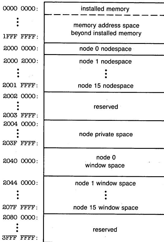
Figure B.16 VAX 8200 Physical Address Space
