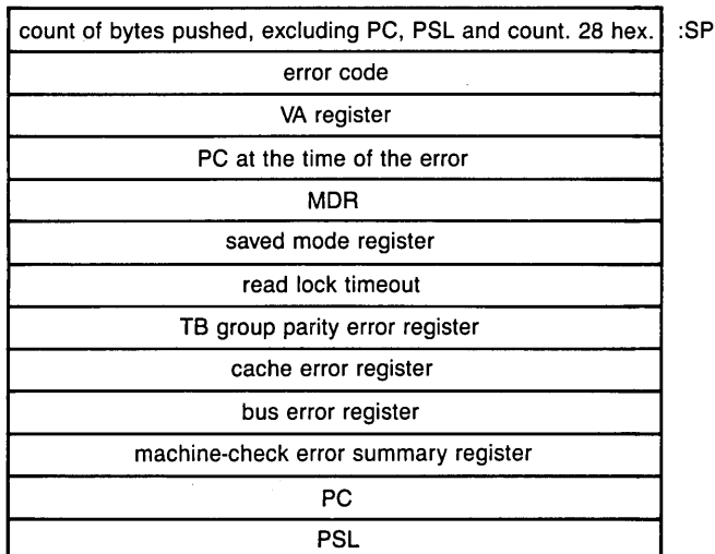
Figure B.12 VAX-11/750 Machine-Check Stack Frame
