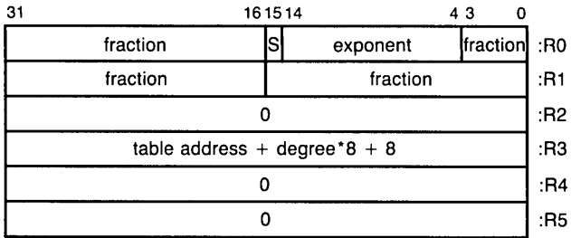
Figure 3.5 POLYG Result Register
