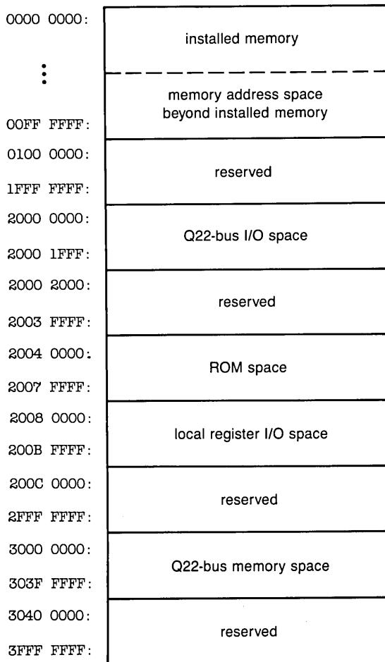
Figure B.4 MicroVAX II Physical Address Space
