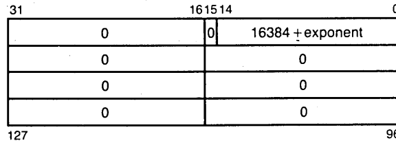
Figure 2.4 Interpretation of a Literal
