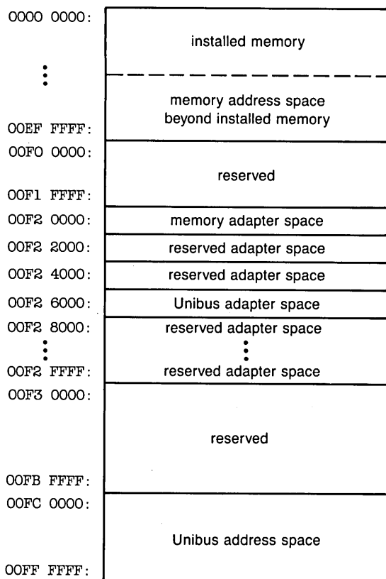
Figure B.7 VAX-11/730 Physical Address Space
