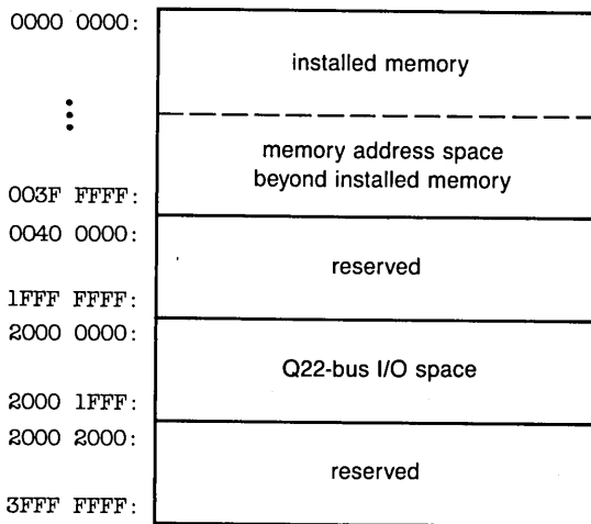
Figure B.1 MicroVAX I Physical Address Space
