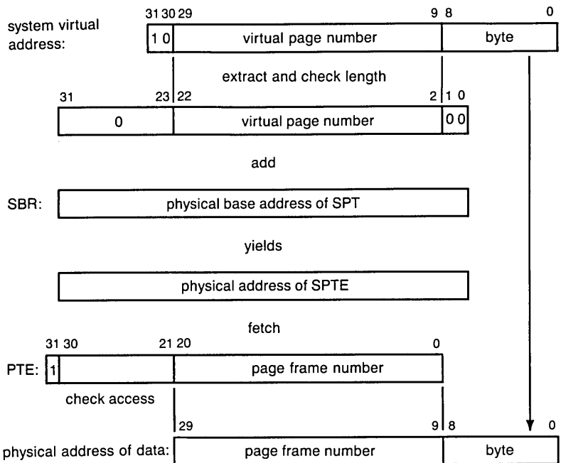
Figure 4.7 System Virtual Address to Physical Translation
