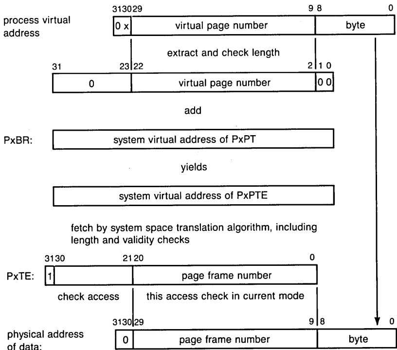
Figure 4.10 Process Virtual Address to Physical Address Translation
