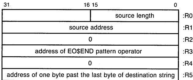
Figure 3.9 EDITPC Control Block
