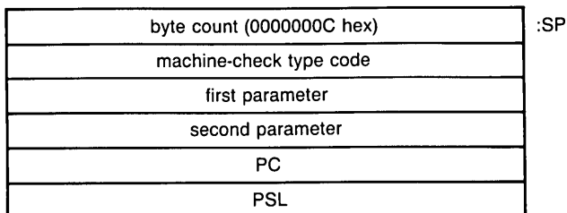
Figure B.3 MicroVAX I Machine-Check Stack Frame
