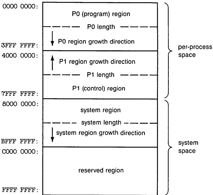
Figure 4.1 Virtual Address Space
