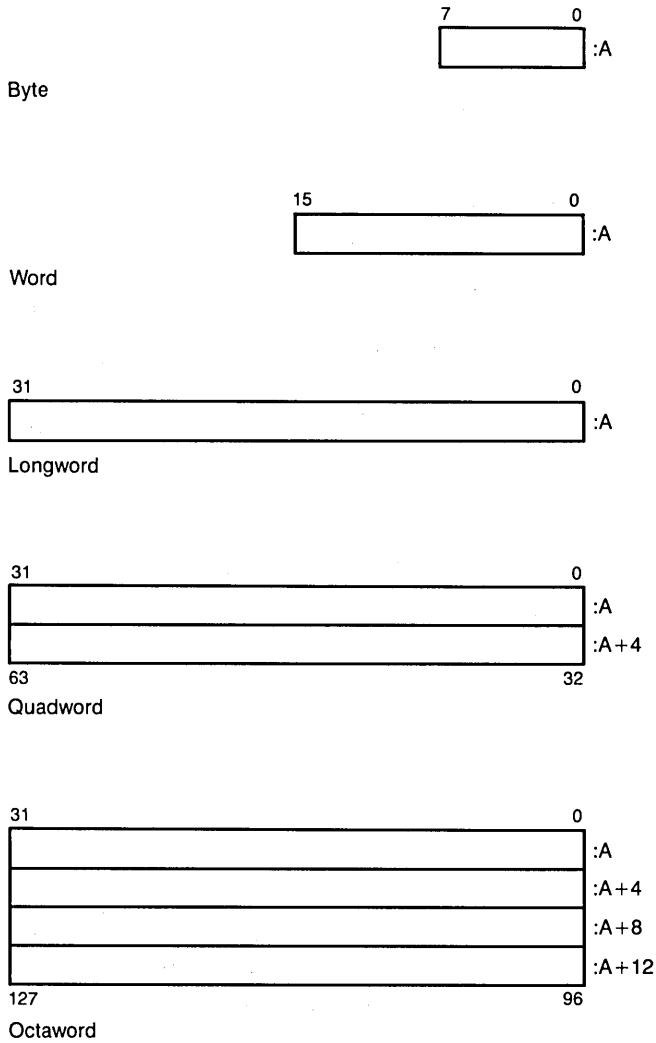
Figure 1.1 Data Types
