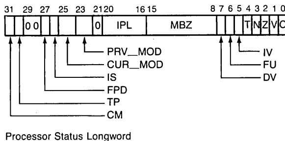
Figure 1.10 The Processor State
