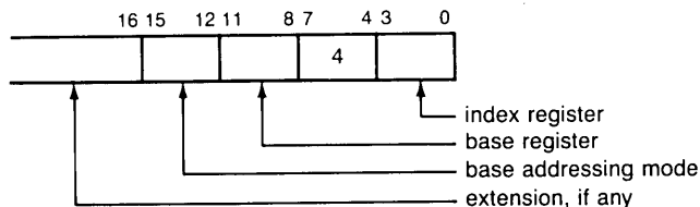
Figure 2.5 Indexed Address Mode Specifier and Extension
