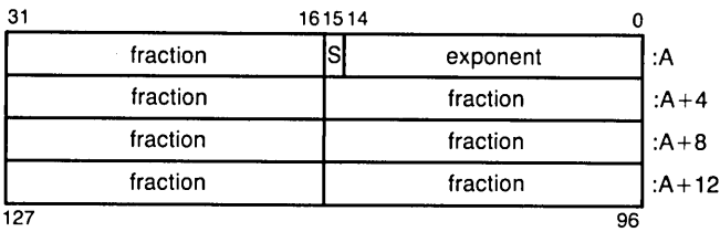
H__floating Data Type (Extended-Range Quadruple Precision)
