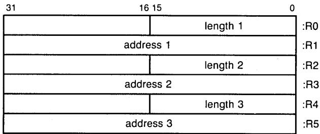
Figure 3.7 Character-String Instruction Control Block
