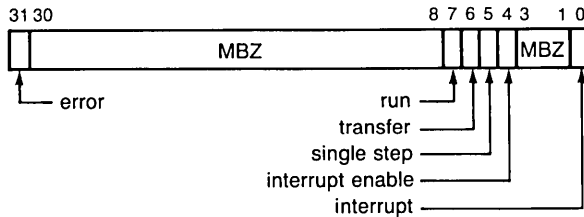
Interval Clock Control and Status (ICCS)
