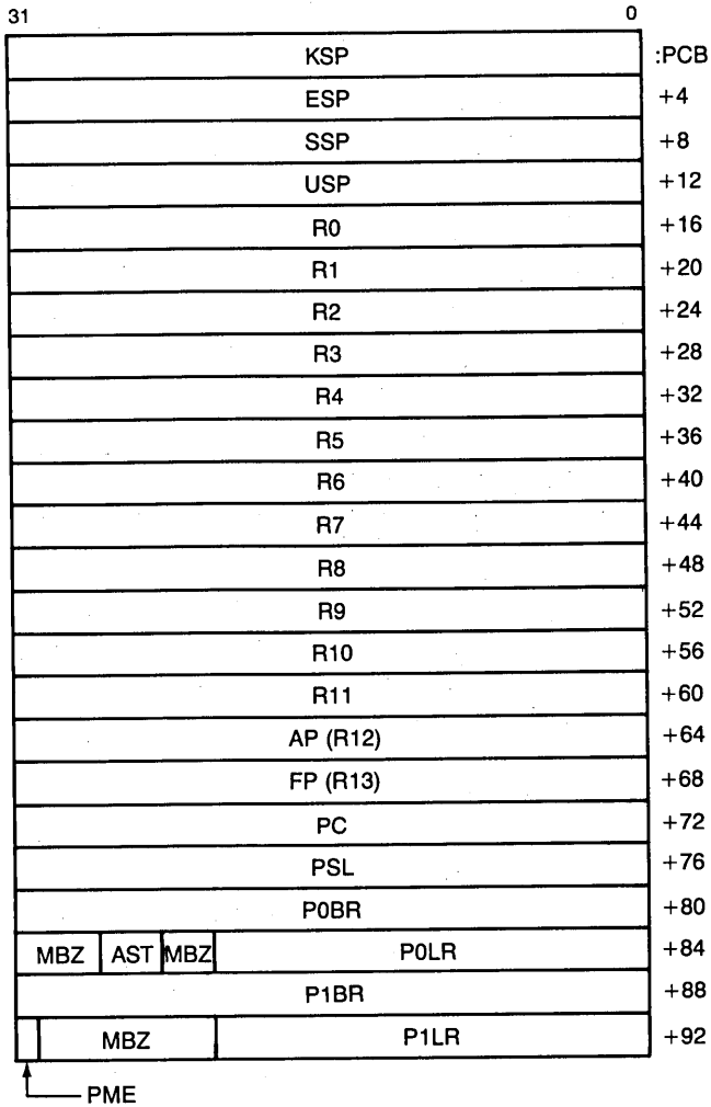
Figure 6.1 Process Control Block (PCB)
