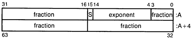
G__floating Data Type (Extended-Range Double Precision)
