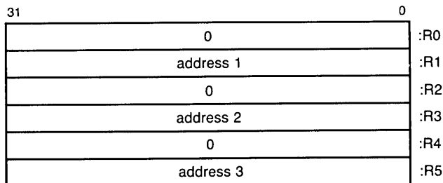
Figure 3.8 Decimal-String Instruction Control Block
