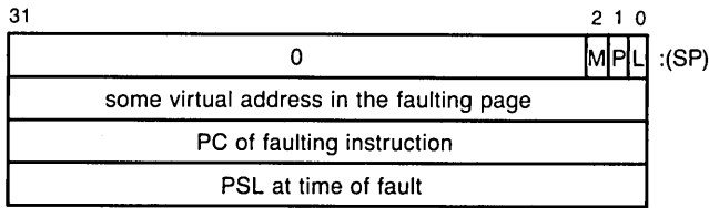
Figure 4.12 Memory Management Fault Stack Frame
