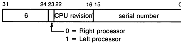
Figure B.23 VAX 8800 System Identification Register (SID)
