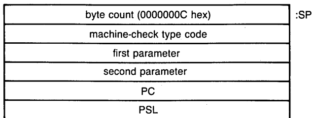
Figure B.9 VAX-11/730 Machine-Check Stack Frame
