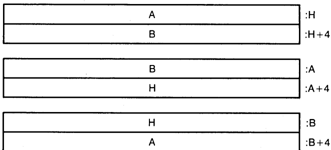
An Absolute Queue with Two Entries
