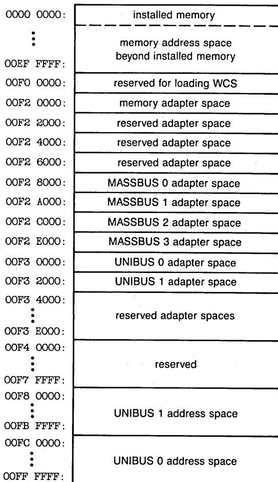
Figure B.10 VAX-11/750 Physical Address Space
