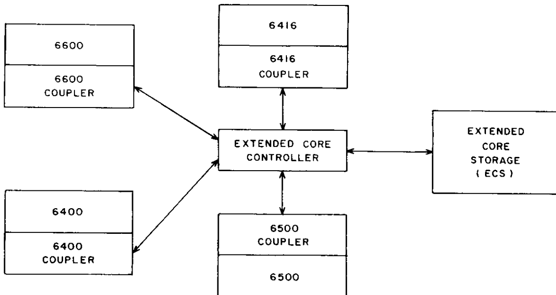
Figure 1-1. Typical Extended Core Storage Configuration
