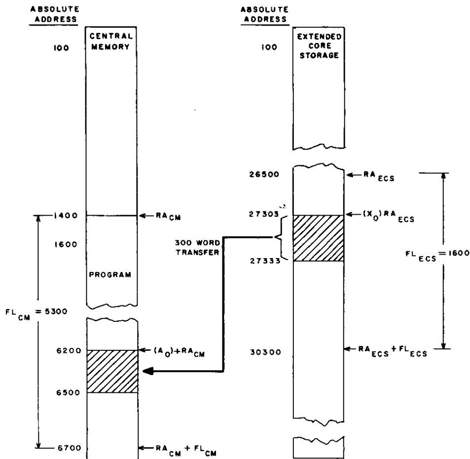
Figure 2-2. Memory Map (Read ECS Example)
