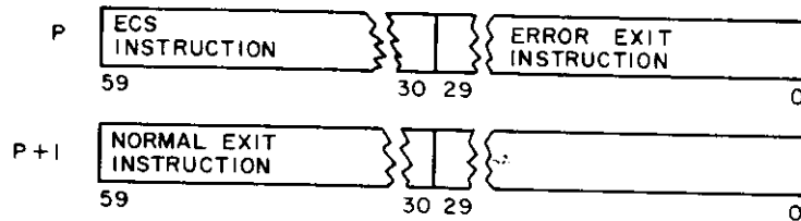
Figure 2-1. Instruction Locations
