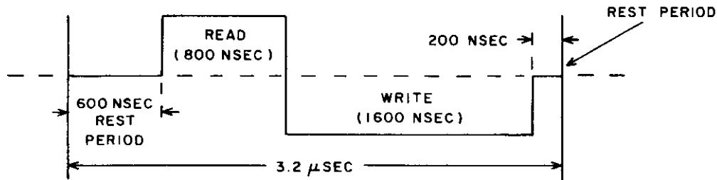
Figure 1-3. ECS Read/Write Cycle
