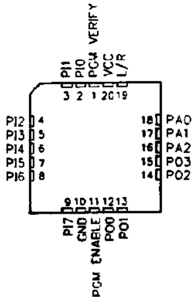
(TOP VIEW)
