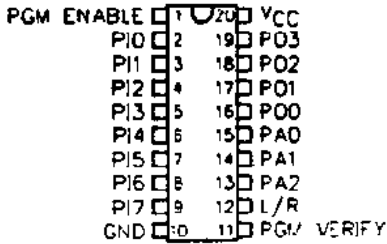
PRODUCT TERMS 0 THRU 31 (TOP VIEW)
